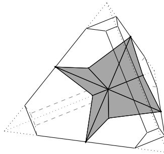
Figure 3: K \subset K^f \subset P when W = D_\infty \times D_\infty and P = \Delta^3
