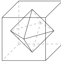
Figure 1: (\Lambda, S) –chamber when \Lambda is the boundary complex of an octahedron
