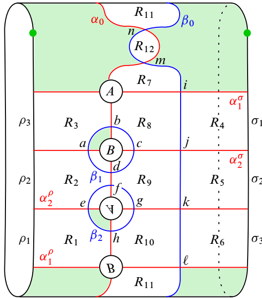
Figure 15: A Heegaard diagram \mathcal{H}_{SG} for the self gluing bimodule
