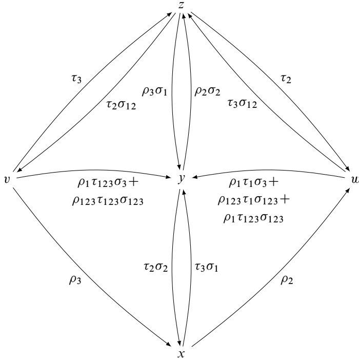
Figure 14: \widehat{\text{CFD}}^3(\mathcal{Y}_{\mathcal{P}}) in the middle \text{spin}^c -structure after canceling the differential from t to s in \widehat{\text{CFD}}^3(\mathcal{H}')
