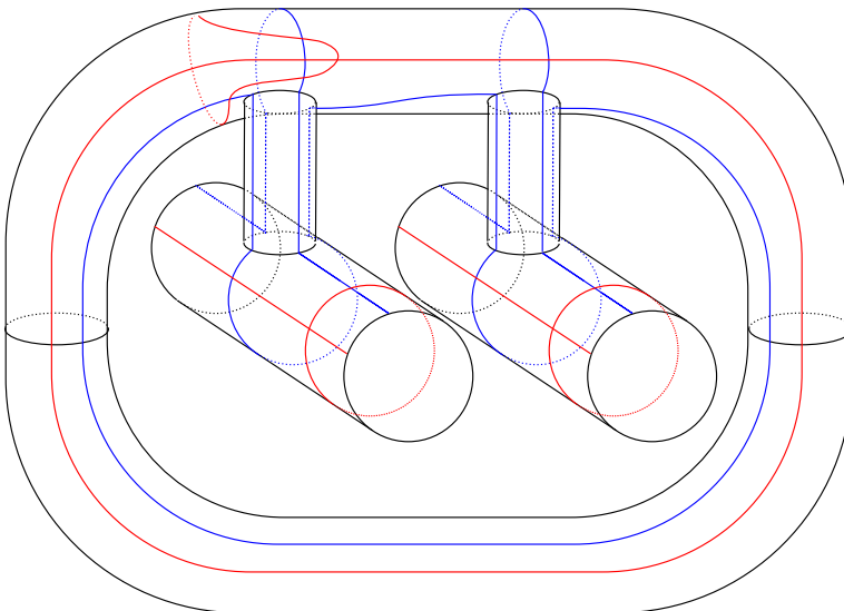
Figure 5: The diagram is easier to read and manipulate if we redraw the outer torus.
