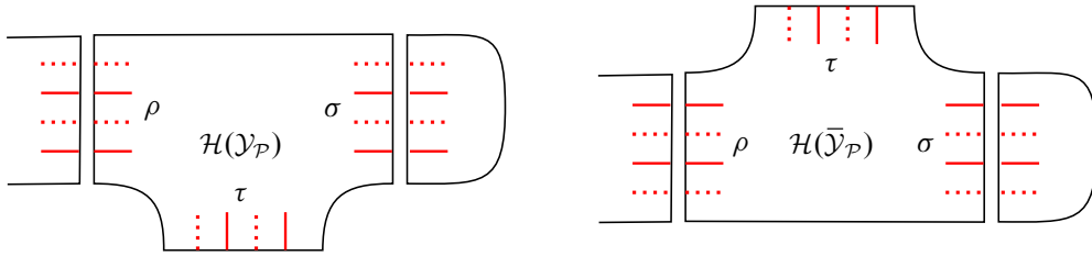
Figure 23: The fiber direction can be changed by extending at a boundary with \mathcal{Y}_{\mathcal{P}} or \overline{\mathcal{Y}}_{\mathcal{P}} and an appropriate solid torus. Dotted lines indicate \alpha arcs which are fibers. The arrangement on the left changes the fiber from \alpha_1 to \alpha_2 , while the arrangement on the right does the opposite.
