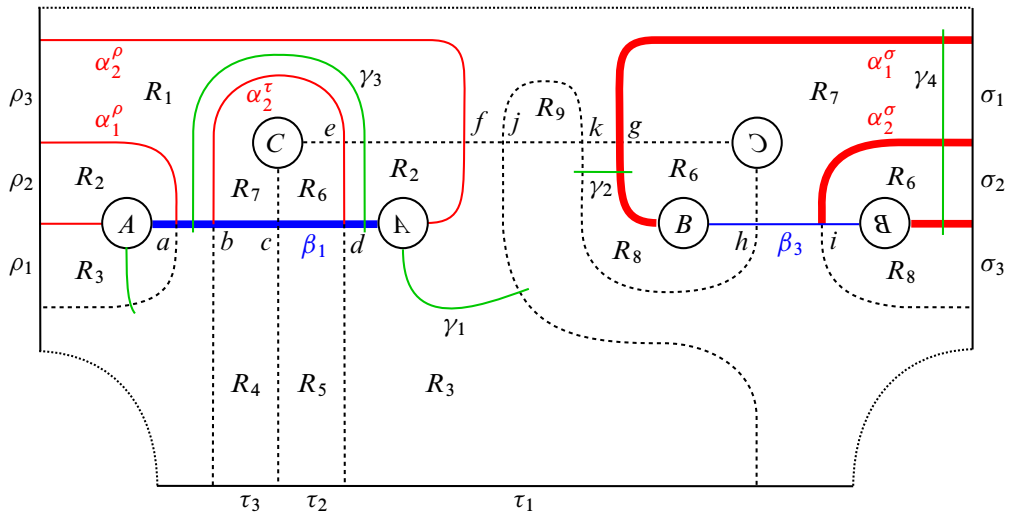
Figure 9: We choose a complex structure J for which the four \gamma arcs are very short and the bold \alpha and \beta segments are very long relative to the thin, solid \alpha and \beta segments.
