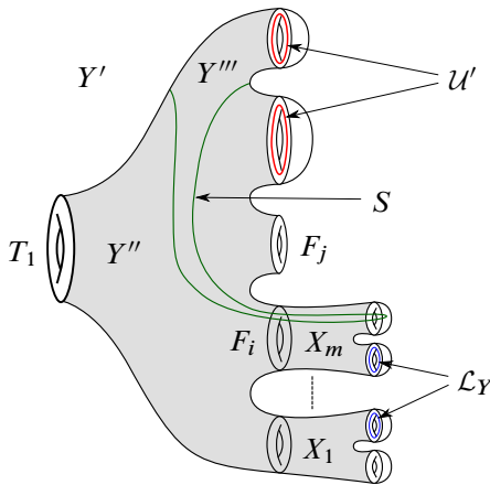
Figure 6: Y'(\alpha_{Y'})
