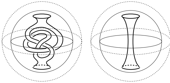
Figure 3: Unknotting in a ball
