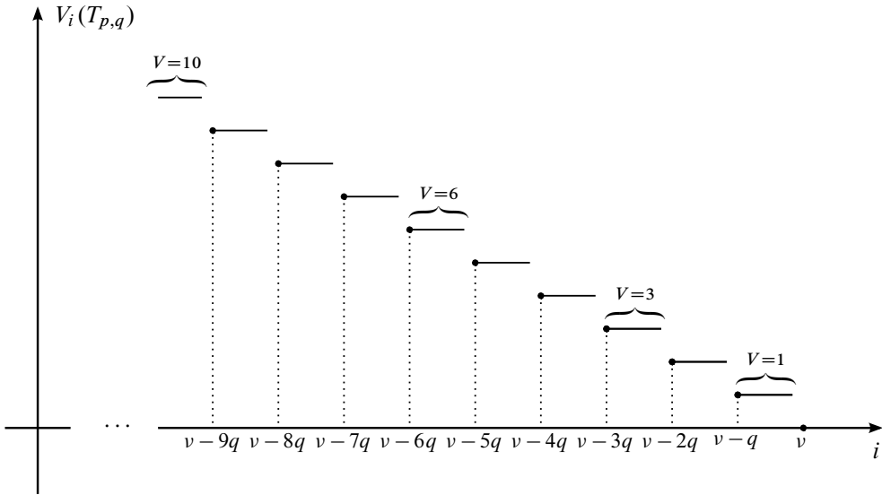
Figure 2: A portion of the graph of the function V(\cdot) , under the assumption p > 9q . We let v = v(T_{p,q}) = \frac{(p-1)(q-1)}{2} .
