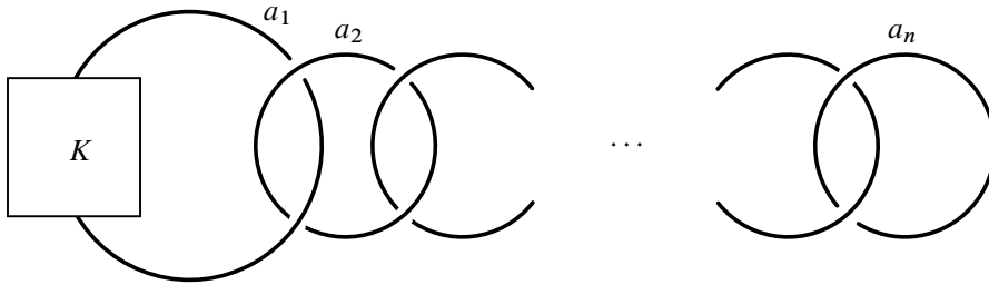
Figure 1: The integral surgery picture for \frac{p}{q} -surgery along K , where \frac{p}{q} = [a_1, \dots, a_n]^-
