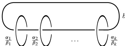
Figure 3: A surgery description for the Seifert fibred manifold Y(b; \alpha_1/\beta_1, \dots, \alpha_k/\beta_k)
