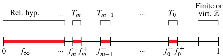
Figure 4: Prevalence of thickness along the “spectrum” of densities p(n) , if the answer to Question is positive; bold intervals are where, conjecturally, W_\Gamma is as thick of a specified order.
