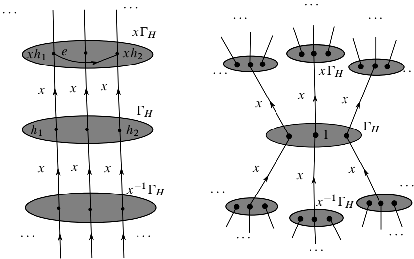
Figure 1: H \times \mathbb{Z} (left) and H * \mathbb{Z} (right)
