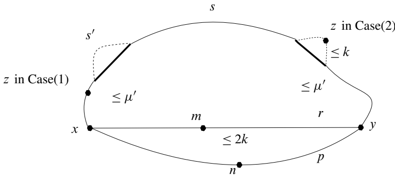
Figure 3: Theorem 2.19
