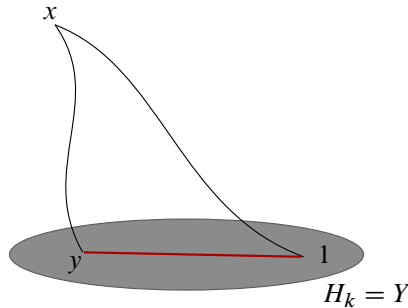
Figure 10: Case 2
