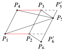
Figure 18: Cylinder with bounded circumference and area at least \frac{1}{2} in a slit torus
