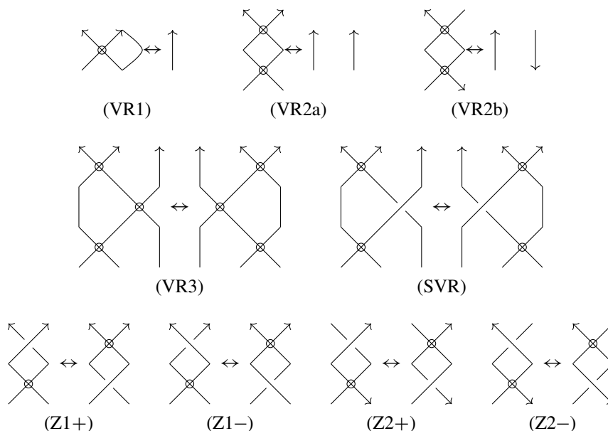
Figure 15: Virtual Reidemeister moves and Z-moves
