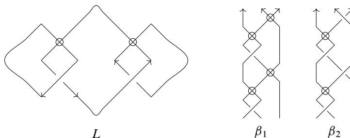
Figure 23: A connected sum of two virtual Hopf links, L , and two braid presentations of L
