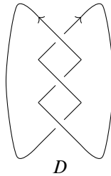
Figure 7: Diagram of the left-handed trefoil knot
