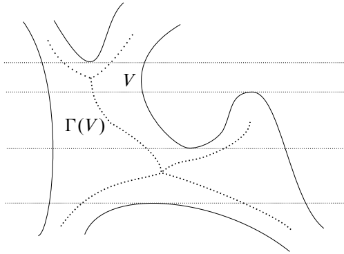
Figure 2: Embedding of \Gamma(V) into V
