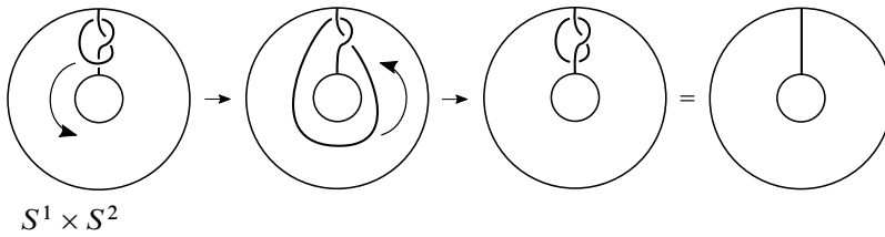
Figure 1: The “light bulb” move in S^1 \times S^2
