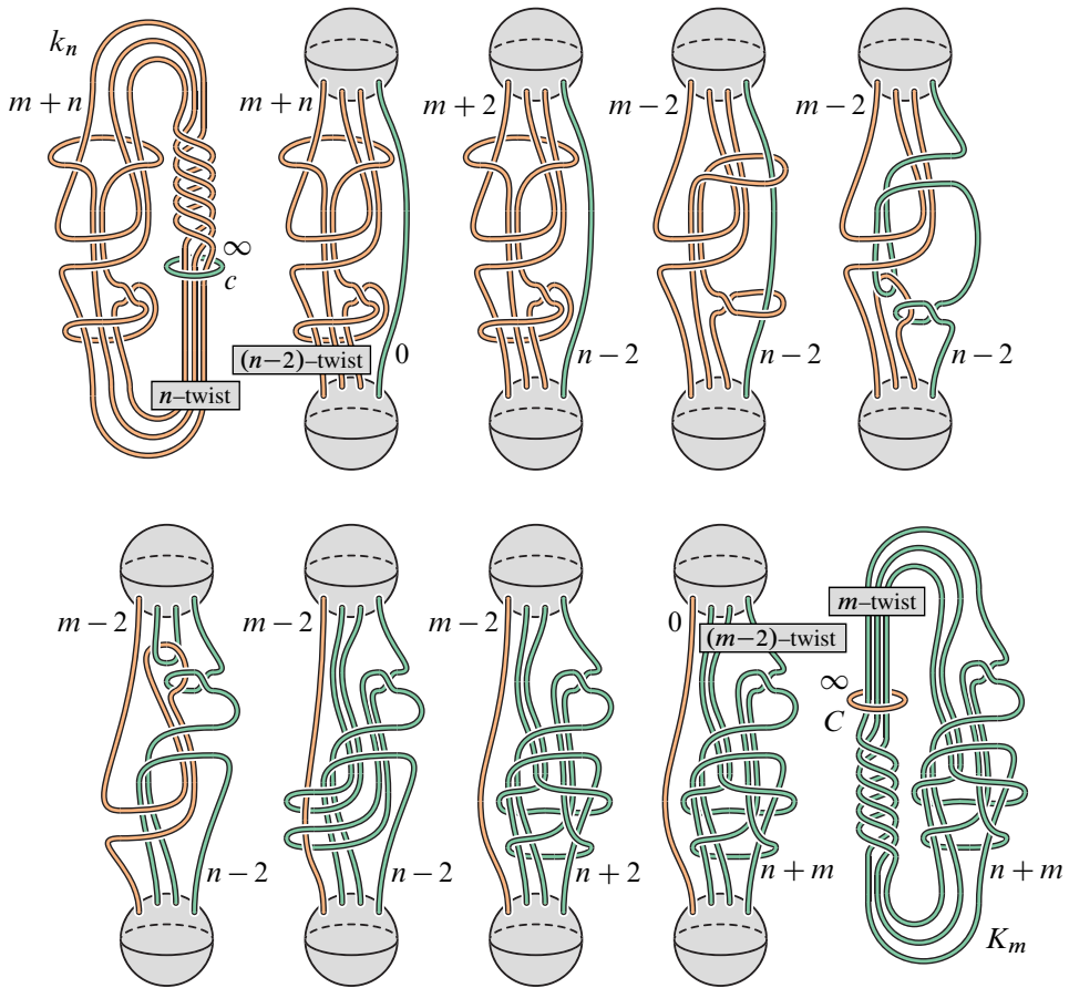
Figure 7: Two families of knots \{k_n\} and \{K_m\} such that k_n(m+n) = K_m(n+m)
