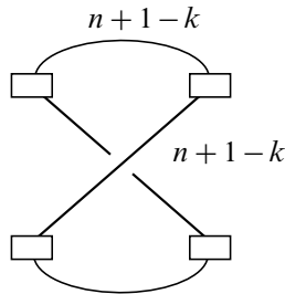
Figure 18: U^{n+1-k}
