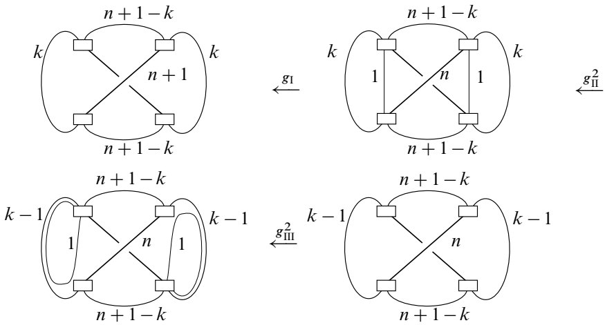
Figure 17: The sequence of local transformations reducing k
