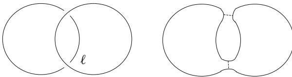
Figure 3: A non- A -adequate diagram of the 2-component unlink and its all- A state. A crossing corresponding to a one-edged loop in s_A(D) is marked \ell .
