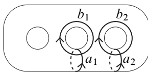
Figure 7: The curves generating H_1(T^4; \mathbb{Z})
