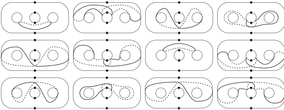
Figure 6: Vanishing cycles of a holomorphic genus-3 pencil on T^4 due to Smith. From left to right, the curves (top row) \tilde{c}_{12}, \tilde{c}_{11}, \tilde{c}_{10}, \tilde{c}_9 ; (middle row) \tilde{c}_8, \tilde{c}_7, \tilde{c}_6, \tilde{c}_5 ; (bottom row) \tilde{c}_4, \tilde{c}_3, \tilde{c}_2, \tilde{c}_1 .
