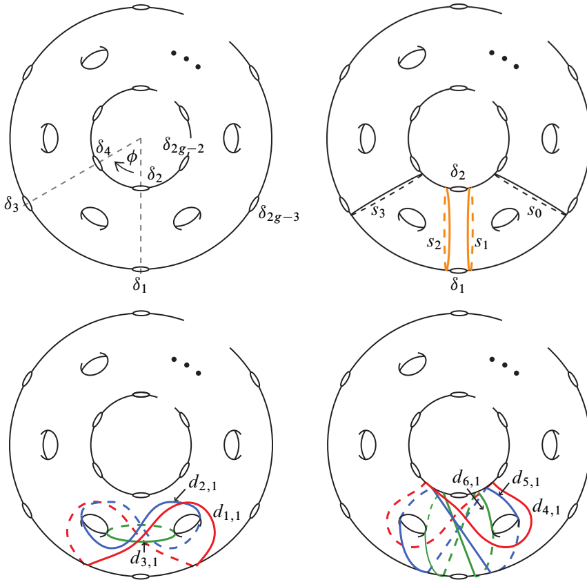
Figure 15: Construction of a generalization of Smith's pencil. Top: the surface \Sigma_g^{2g-2} and the rotation \phi (left) and the curves s_1 = s_{2g-1}, s_2, s_3, s_0 = s_{2g-2}, \delta_1 and \delta_2 (right). Bottom: the curves d_{1,1}, d_{2,1}, d_{3,1} (left) and the curves d_{4,1}, d_{5,1}, d_{6,1} (right).
