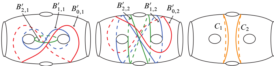
Figure 13: Modified lift of Matsumoto's factorization
