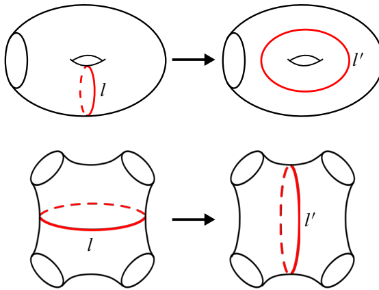
Figure 1: Above: An S-move in the pants complex. Below: An A-move in the pants complex.
