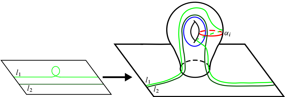
Figure 8: Resolving a Reidemeister 1 move to change the surface framing of l_1 by 1. Parallel curves such as l_2 can be sent over the stabilizing surface without twisting about \alpha_i to preserve the surface framing.
