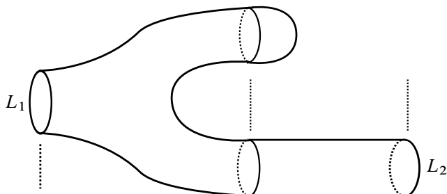
Figure 12: Death cobordism
