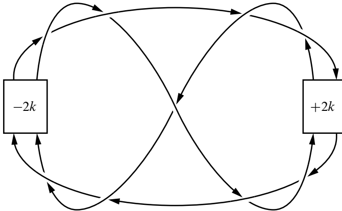
Figure 1: A diagram of L^k . For k = 0 we have the link L^9_{40} .
