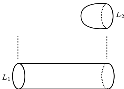
Figure 8: Birth cobordism
