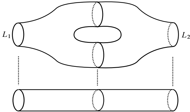
Figure 7: Torus cobordism
