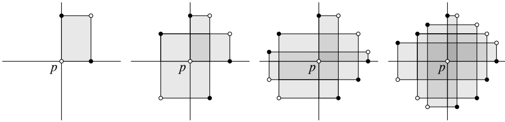
Figure 11: Some of the snail-like domains \mathcal{SL}(x, z, p) ; the coordinates of x and z are represented by the white and black circles.
