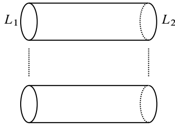
Figure 4: Identity cobordism
