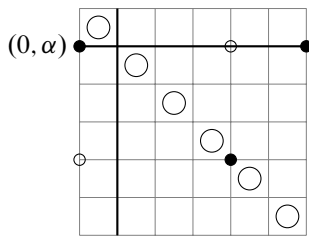
Figure 15: The state y \in I(D) is marked with the black circles.
