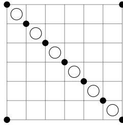
Figure 14: We denote by x the grid state in the picture.
