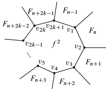
Figure 2: A 2-face f^2 with an odd number of vertices
