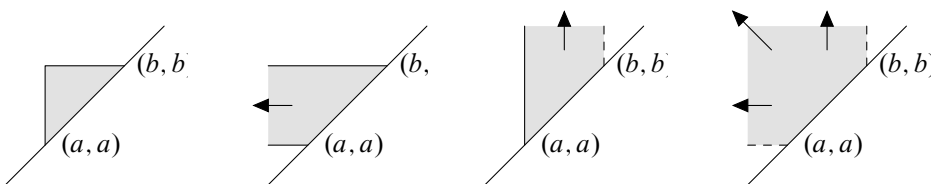
Figure 14: Four almost-blocks that are not blocks
