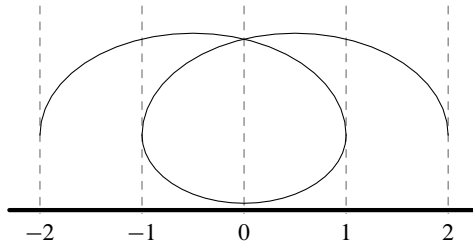
Figure 5: The immersed curve T of Examples 4.6 and 4.10
