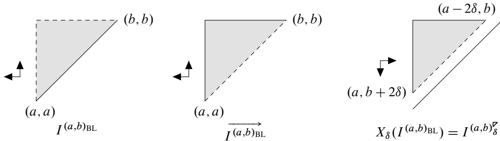
Figure 13: Applying X_\delta(-) to I^{(a,b)BL}
