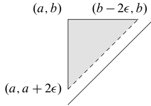
Figure 8: An interval (a, b)^\nabla_\epsilon
