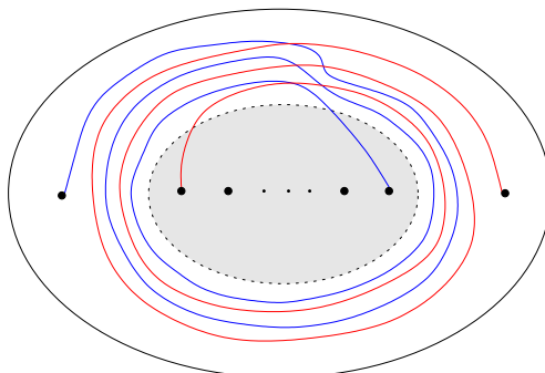
Figure 3: The monodromy of the braid \beta is supported inside the shaded disk. The two stabilizing arcs twist around.
