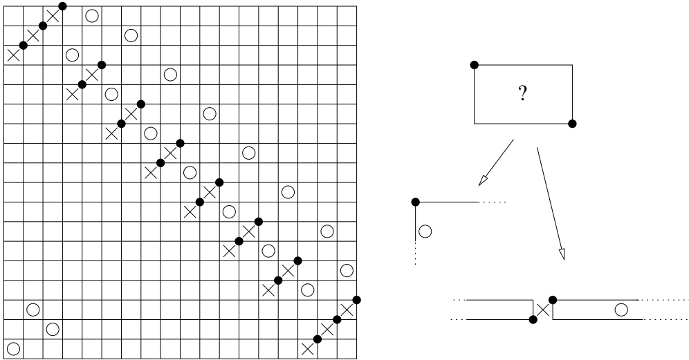
Figure 5: The cycle \hat{\theta} (left) and looking for empty rectangles (right)
