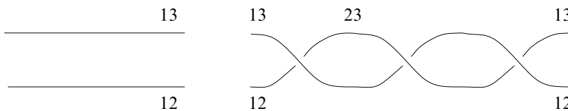
Figure 7: Modification of the branch locus for a 3-fold simple cover
