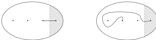
Figure 2: Markov stabilization \beta \mapsto \beta\sigma_m (left) and stabilization along an arbitrary arc (right)
