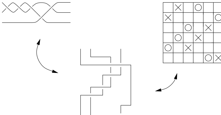
Figure 1: Braids and grid diagrams. The middle picture shows a braid running from bottom to top, constructed from the grid diagram on the right. The picture on the left shows the same braid running from left to right; the braid closure is braided around the (vertical) z -axis and represents a transverse link in (\mathbb{R}^3, \ker(dz + r^2 d\phi)) .
