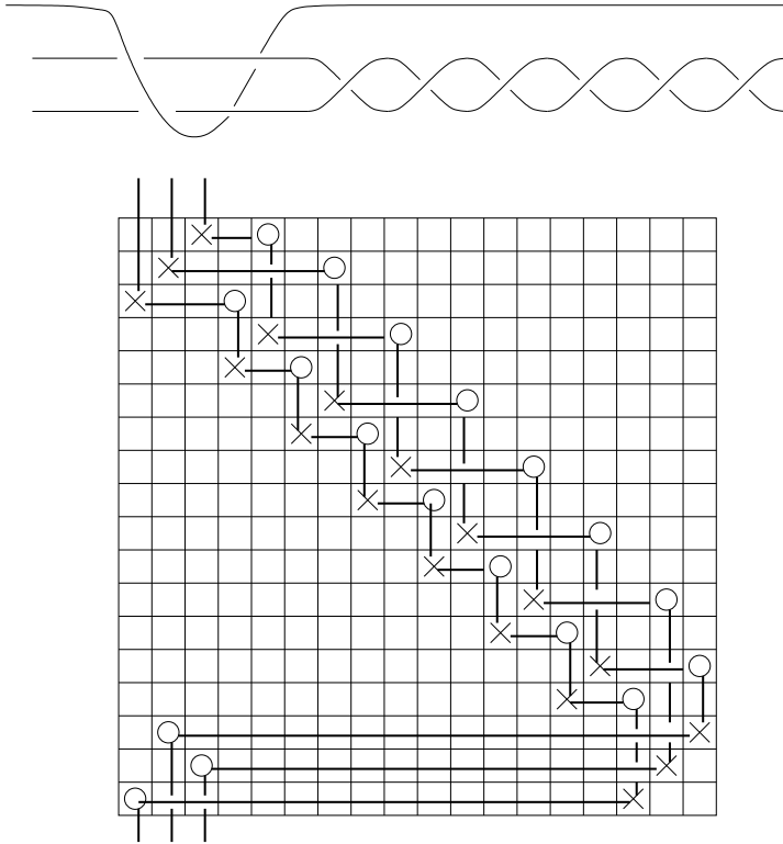
Figure 4: A grid diagram for \sigma_1\sigma_2\sigma_2\sigma_1\sigma_2^{-k}
