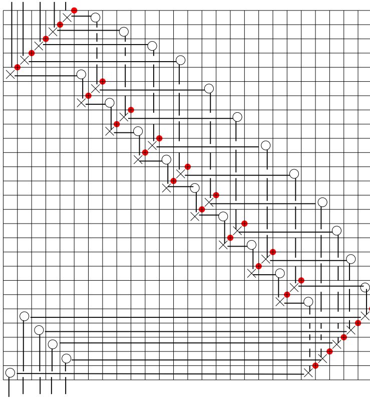
Figure 6: The cycle \hat{\theta} for a braid \beta'_{n,k} = \beta_{n,k} with n = 5 and k = 2
