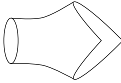
Figure 6: A trigon
