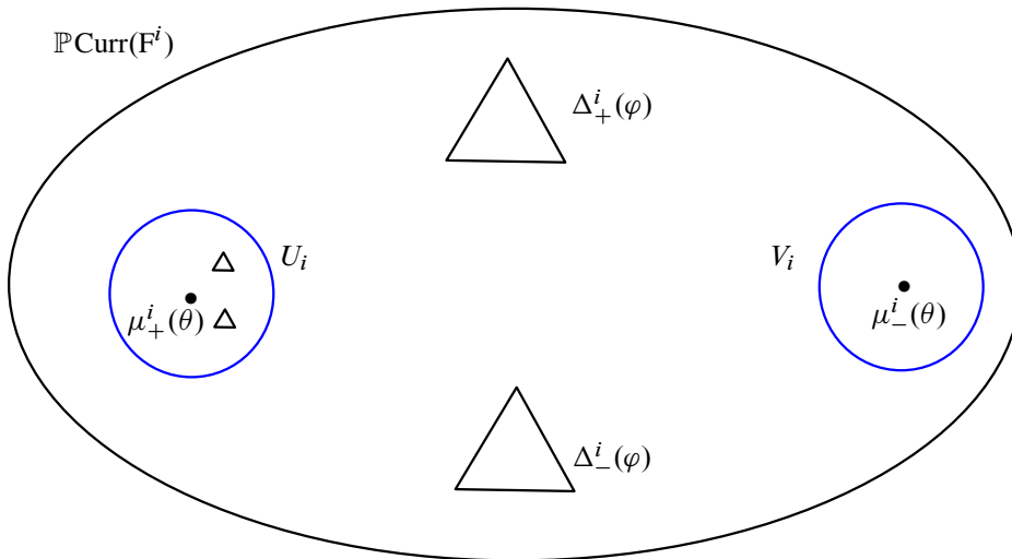
Figure 1: Dynamics on \mathbb{P}\text{Curr}(F^i)
