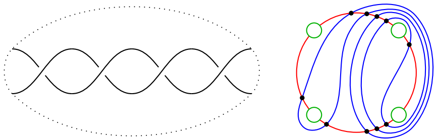
Figure 14: Illustration of Example 4.3. Left: a rational tangle obtained from the 1-crossing tangle in Figure 13, left, by three Dehn twists on the right. Right: a genus 0 Heegaard diagram for the left tangle.
