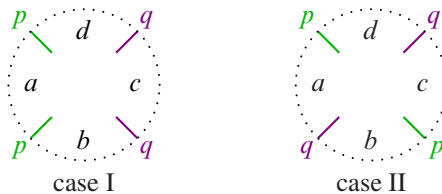
Figure 19: The two cases for Theorem 6.7.
