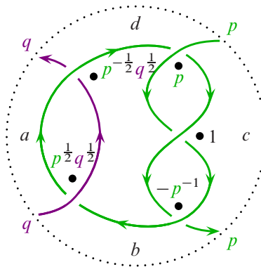
Figure 6: A Kauffman state of a 4-ended tangle.
