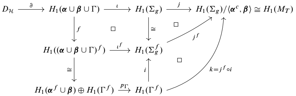
Figure 15: Diagram for the definition of A^f in Definition 5.4. The maps \iota , \iota^f , i and j are induced by inclusions, and p_\Gamma is the projection onto the second summand.
