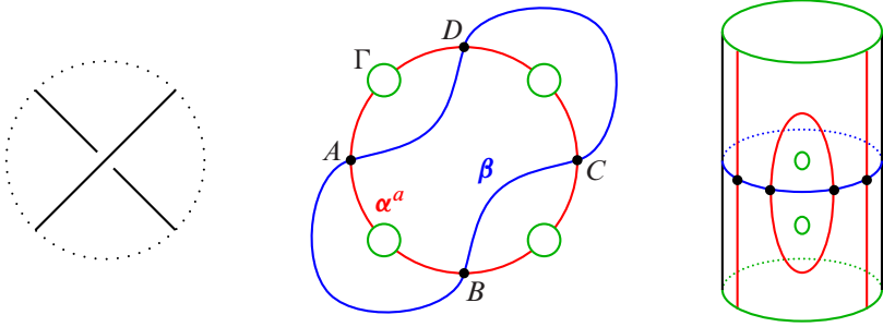
Figure 13: The two building blocks of tangle Heegaard diagrams in Example 4.2. Left: a single crossing tangle. Centre: a Heegaard diagram for the tangle on the left. Right: a ladybug; this terminology is taken from [6, Figure 9c].
