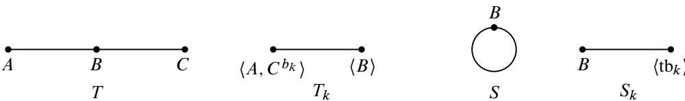
Figure 2: Examples showing the impossibility to extend continuously the natural intersection pairing in the relative setting.
