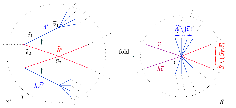
Figure 3: (ii) \iff (iii) in the case of a fold.
