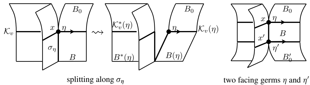
Figure 11: The splitting process.
