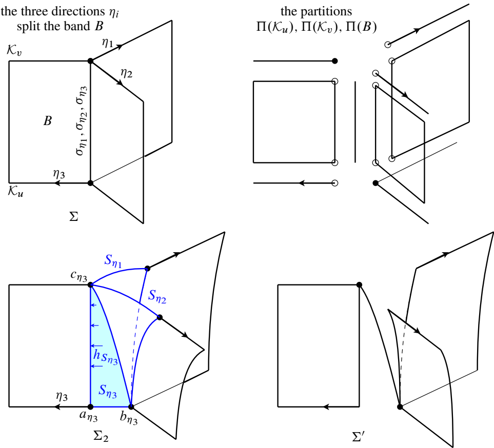
Figure 12: \Sigma , the partitions, \Sigma_2 and \Sigma' .
