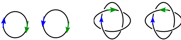
Figure 11: Relative orientations of the reconnection sites: an unknotted chain with two sites in direct repeats (far left) and an unknotted chain with two sites in inverted repeats (second from left). T(2, n) torus links with parallel orientation of the strands and linking number +n/2 (second from right) and antiparallel orientation of the strands and linking number -n/2 (far right).
