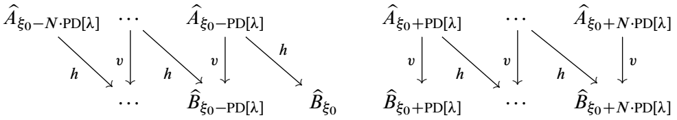
Figure 7: The kernel of the quotient from \widehat{X}_{\xi_0}^N to \widehat{A}_{\xi_0} . The left summand (respectively right summand) corresponds to Q_- (respectively Q_+ ).
