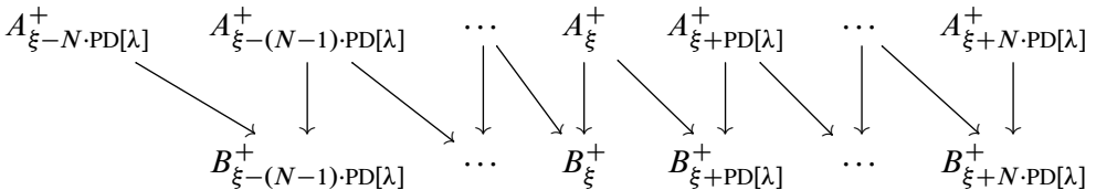
Figure 5: The truncated mapping cone \mathbb{X}_{\xi}^{+, N} computing the complex \text{CF}^+(Y_{\lambda}(K), G_{Y_{\lambda}(K), K_{\lambda}}(\xi)) in the case that |H_1(Y_{\lambda}(K))| \equiv -1 \pmod{3} .
