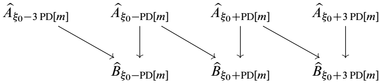
Figure 8: When k = 1 , up to homotopy, \widehat{\mathbb{X}}_{\xi_0+PD[\theta]} splits off this summand.
