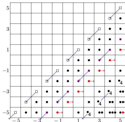
Figure 2: The E^1 -page of the Atiyah–Hirzebruch spectral sequence for -5 \leq s \leq 5 and -5 \leq t \leq 5 with d^1 -differentials included. A \square represents \mathbb{Z}_{(2)}[\tau] , a \bullet represents \mathbb{F}_2[\tau] , a violet \bullet represents
