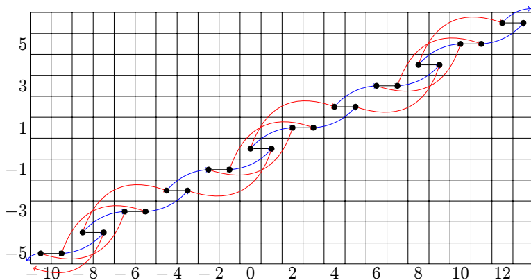
Figure 1: This depicts the continuous motivic cohomology H_c^{i,j}(\Sigma^{1,0}\underline{L}_{-\infty}^\infty) for -11 \leq i \leq 12 and -5 \leq j \leq 6 . The horizontal axis is topological degree and the vertical axis is motivic weight. A bullet represents \mathbb{M}_2 , ie it represents an infinite tower of \mathbb{F}_2 's connected by \tau -multiplication extending downwards. The action of Sq^1 is depicted by black horizontal lines between bullets, the action of Sq^2 is depicted by blue curves with horizontal length 2, and the action of Sq^4 is depicted by red curves with horizontal length 4.
