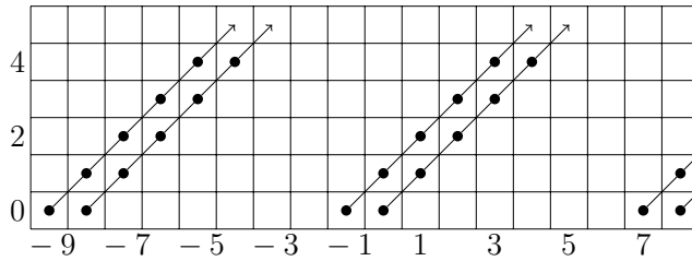
Figure 9: The inverse limit C\tau -linear \overline{H} -based Adams spectral sequence for wko^{t_{gm}C_2} for -9 \leq t-s \leq 8 and 0 \leq s \leq 5 .
