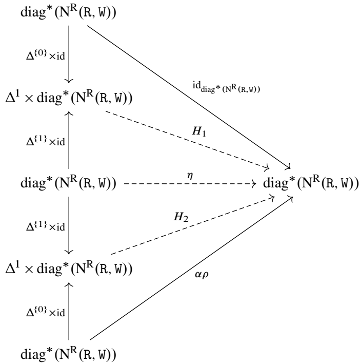
Figure 1: The zigzag of simplicial homotopies in s\mathbf{Set} in the proof of Lemma 4.3.
