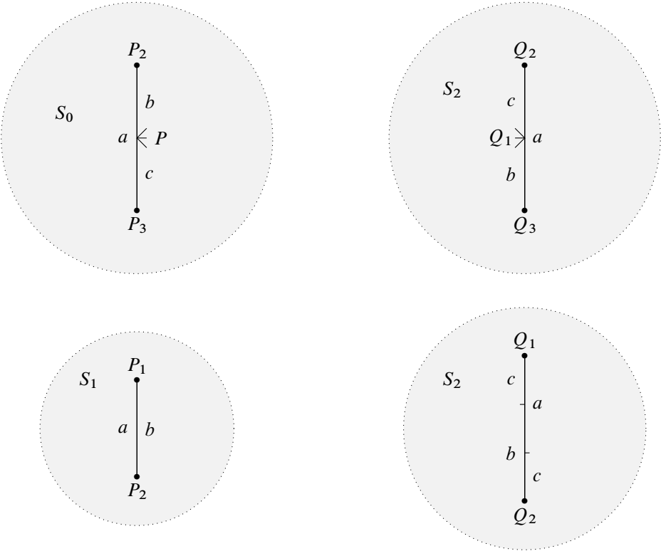
Figure 2: Surfaces in \mathcal{H}(-p, -q, p + q) .
