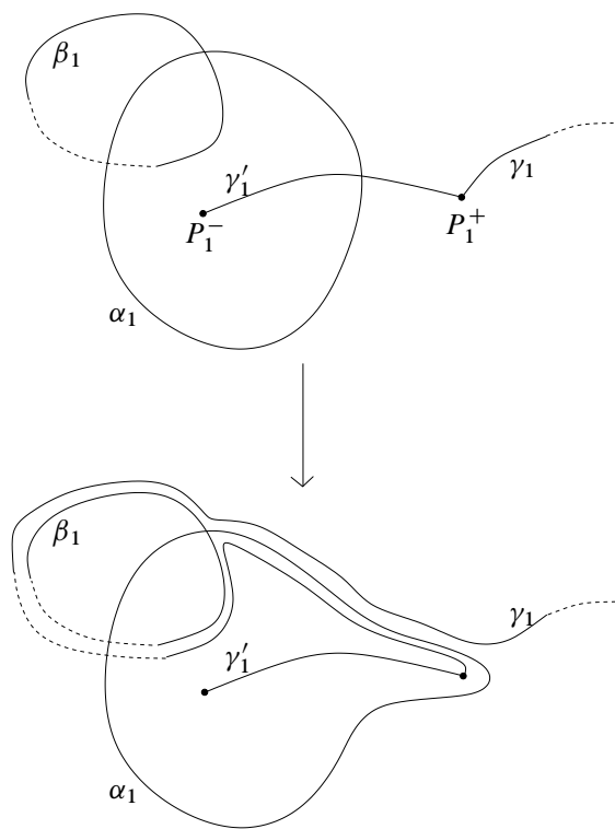
Figure 7: Decreasing the number of intersection points.
