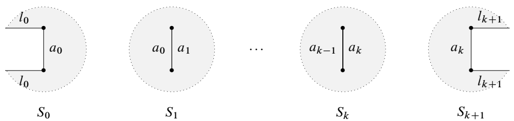
Figure 3: Surface of genus zero in \mathcal{H}(n, p_0, \dots, p_{k+1}) with k poles of zero residues and two poles of nonzero residues.
