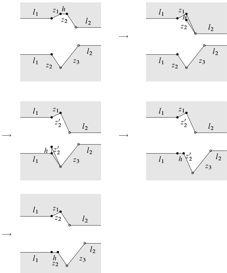
Figure 6: Rotating (clockwise) the hole by \pi .
