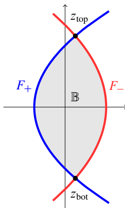
Figure 3: The set \mathbb{B} .
