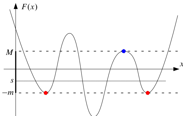
Figure 2: The values M and -m on the plot of a characteristic polynomial.
