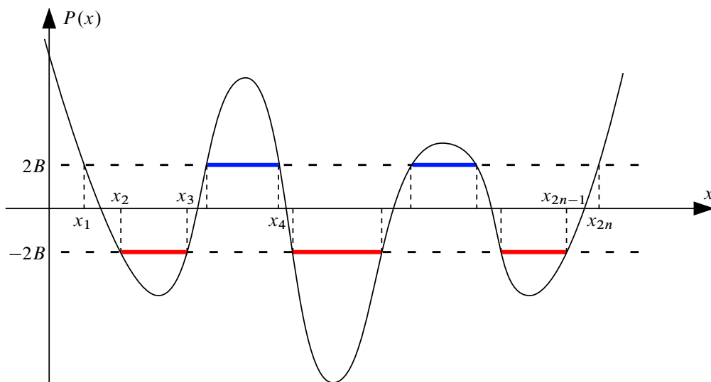
Figure 4: Upper and lower forbidden zones.
