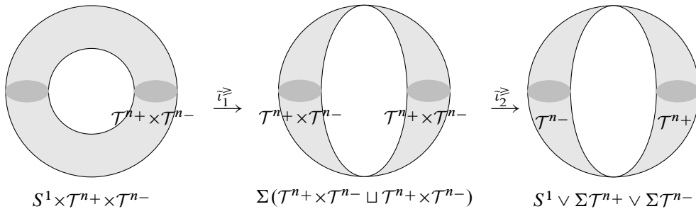
Figure 7: The map \tilde{i}^{\geq} pinches the product S^1 \times (\mathcal{T}^{n+} \times \mathcal{T}^{n-}) at two points of S^1 , then collapses \mathcal{T}^{n+} on the left side and \mathcal{T}^{n-} on the right side.
