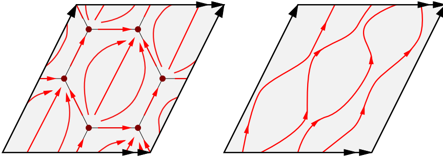
Figure 6: The Toda flow on the level set B = \text{const} of the orbit space Q_{3,\lambda}^0 . Left: the case B = 0 . Right: the case B = \text{const} \neq 0 .
