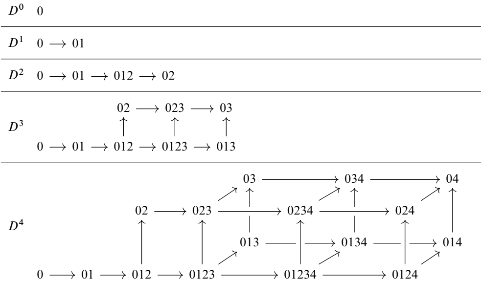
Figure 1: The posets D^n for n \leq 4 .
