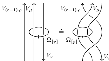
Figure 5: Transparency of f_{[\gamma], \mu, \nu} .
