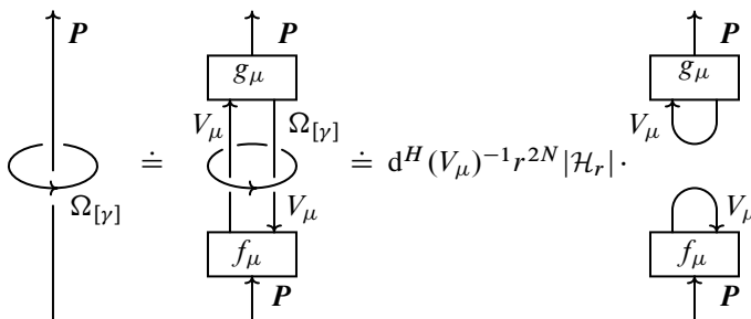
Figure 8: Cutting a \mathbf{P} -colored edge with a Kirby-colored meridian.
