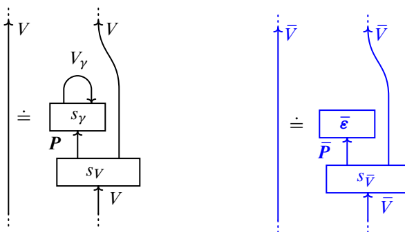
Figure 9: Projective stabilizations on e \subset T and on \bar{e} \subset \bar{T} .
