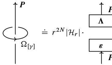
Figure 6: Cutting property for Kirby-colored meridians.
