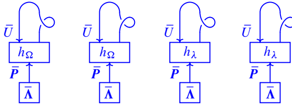
Figure 17: The \bar{\mathcal{C}} -colored ribbon graphs T_{-\Omega}, T_{+\Omega}, T_{-\lambda}, T_{+\lambda} \subset S^3 .
