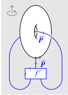
Figure 13: The \bar{\mathcal{C}} -colored ribbon graph T'_{f'} \subset (D^3 \setminus N^3) \cup_{S^2} \bar{D}^3 .
