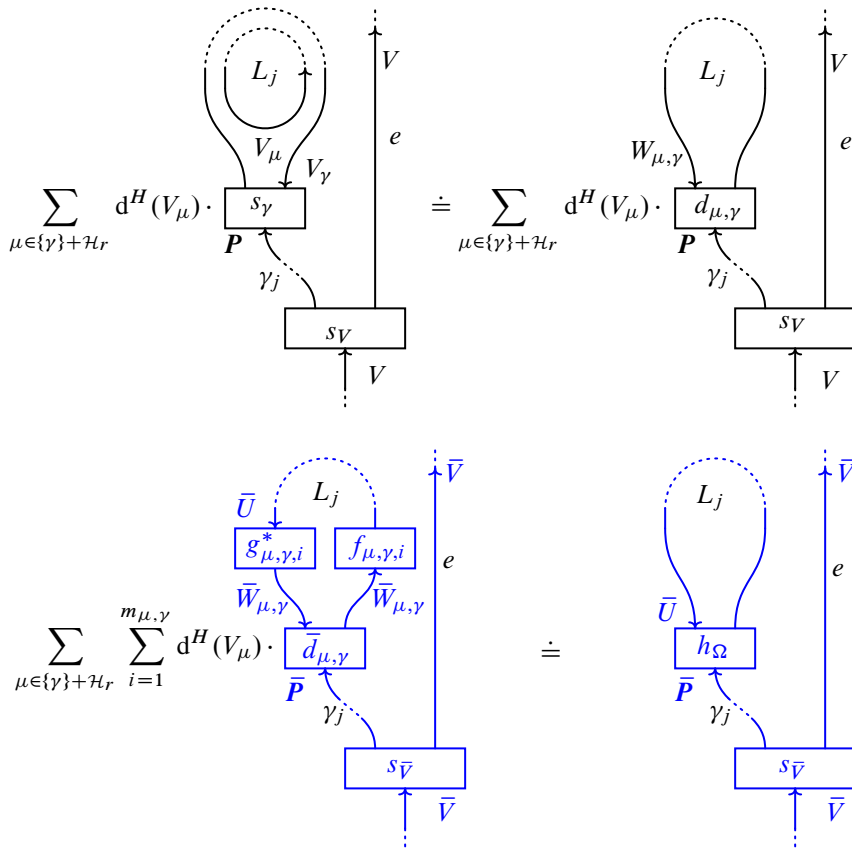
Figure 10: Skein equivalences of \mathcal{C}^H -colored and \bar{\mathcal{C}} -colored ribbon graphs defining (L \cup \bar{T})_{h_\Omega} .
