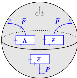
Figure 15: The \bar{\mathcal{C}} -colored ribbon graph T_{D^3} \subset D^3 .
