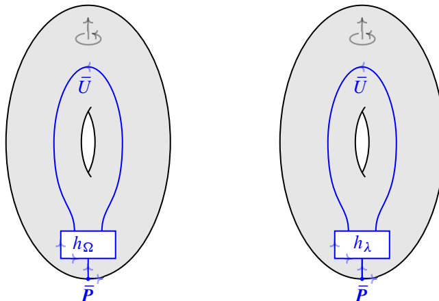
Figure 14: The \bar{\mathcal{C}} -colored ribbon graphs T_{h_\Omega}, T_{h_\lambda} \subset S^1 \times D^2 .
