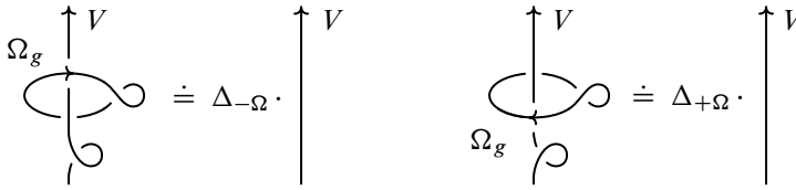
Figure 1: Skein equivalences defining \Delta_{-\Omega} and \Delta_{+\Omega} .
