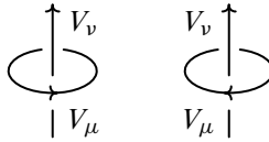
Figure 3: \mathcal{C}^H -colored ribbon graphs T_{\mu,v}^+ and T_{\mu,v}^- .
