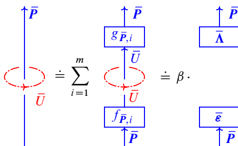
Figure 16: Cutting a \bar{\mathbf{P}} -colored edge with a red meridian.
