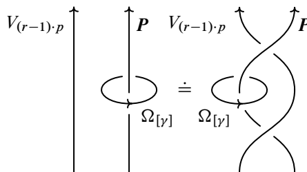
Figure 7: Transparency of h_{[\gamma]} .
