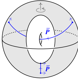
Figure 12: The morphism (\mathbb{D}^3 \setminus \mathbb{N}^3)_{\bar{\mathbf{P}}} of \check{\text{Cob}}_{\bar{\mathcal{C}}} .
