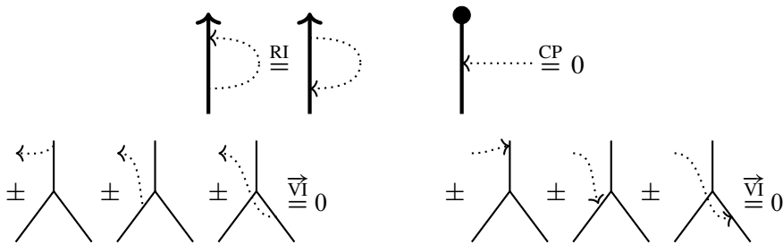
Figure 11: The relations RI, CP, and \overrightarrow{\text{VI}} . Ambiguous strands can be either thick black or thin red. In the \overrightarrow{\text{VI}} relation, signs are positive when the strand of the arrow ending is oriented towards the vertex, and negative otherwise.
