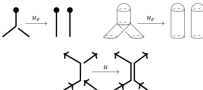
Figure 8: Disc unzip on the top row, strand unzip on the bottom.
