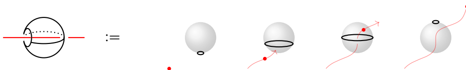
Figure 2: The threaded sphere as a movie of a circle and a point in \mathbb{R}^3 .
