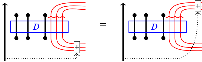
Figure 24: The head invariance property in \mathcal{A}^{sw}(\uparrow^{k_1} \uparrow^{k_2}) .
