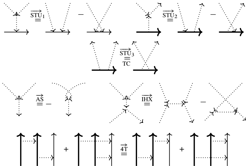
Figure 12: The relations \overrightarrow{\text{STU}} , \overrightarrow{\text{AS}} , \overrightarrow{\text{IH\ddot{X}}} and \overrightarrow{4\text{T}} on \mathcal{A}^{swt} . Ambiguous strands can be either thick black or thin red.
