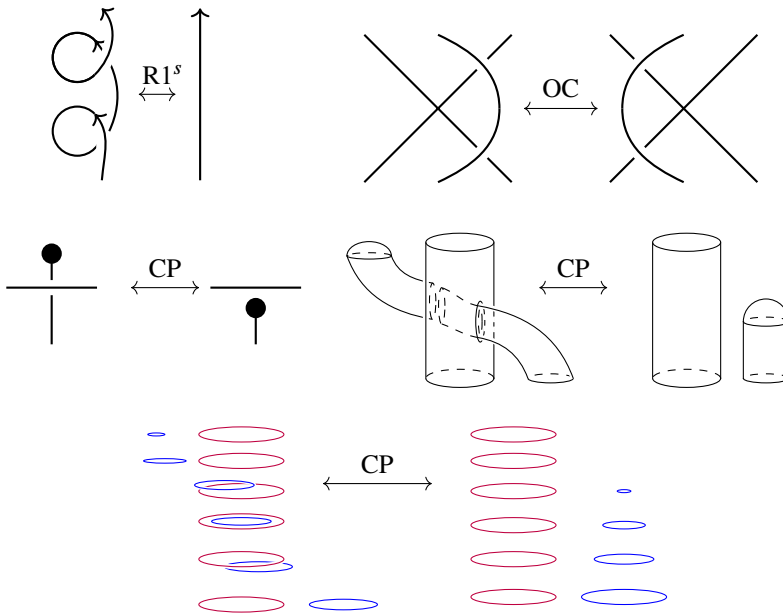
Figure 6: The relations R1^s and OC are shown. CP is explained with broken surface diagrams and as a movie of flying circles.
