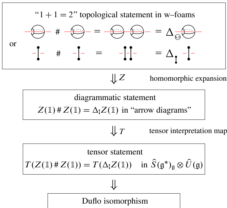
Figure 1: The rough sketch of the proof.
