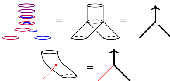
Figure 5: The trivalent vertices of \widetilde{wTF} .
