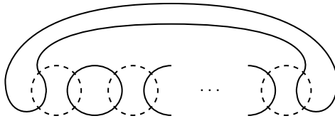
Figure 9: Connectedness diagram for a Montesinos link on n rational tangles with suitably chosen weights.
