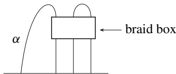
Figure 6: Rational tangle with a distinguished string \alpha .
