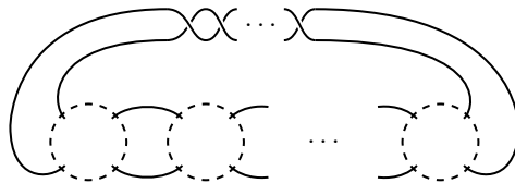
Figure 8: Montsesinos link on n rational tangles.
