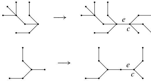
Figure 2: Adding ramification points of valency 4 and 3.
