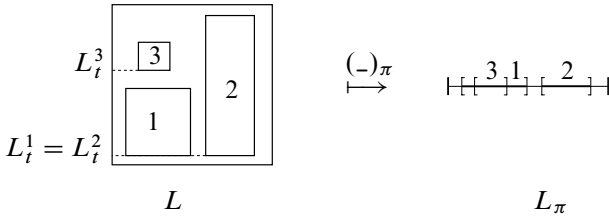
Figure 11: Illustration of the operations (-)_\pi and (-)_t . The permutations \text{id} , (12) and (23) order L .
