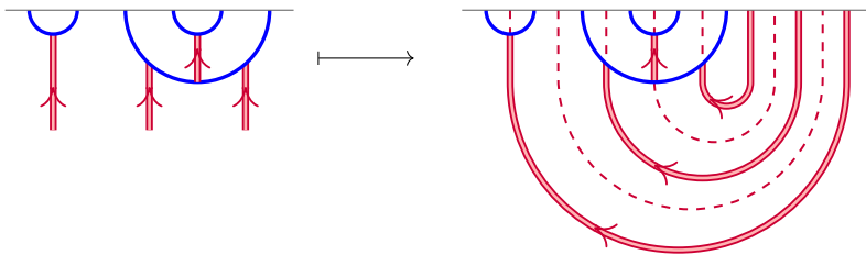
Figure 9: Turning red edges rightwards and to the top produces a cup web from an EST web. There is a natural completion, visualized by dashed arcs, with minima of red cups below all blue ones.
