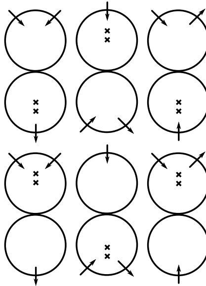
Figure 10: Six possible boundary bubbles. The incoming arrows are inputs and the outgoing ones are outputs.
