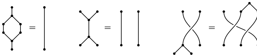
Figure 2: The three key equivalences for strand diagrams, which can occur anywhere inside a strand diagram representing an element of bV . Further equivalences are obtained by combining these, and by rotating and reflecting the one on the right.
