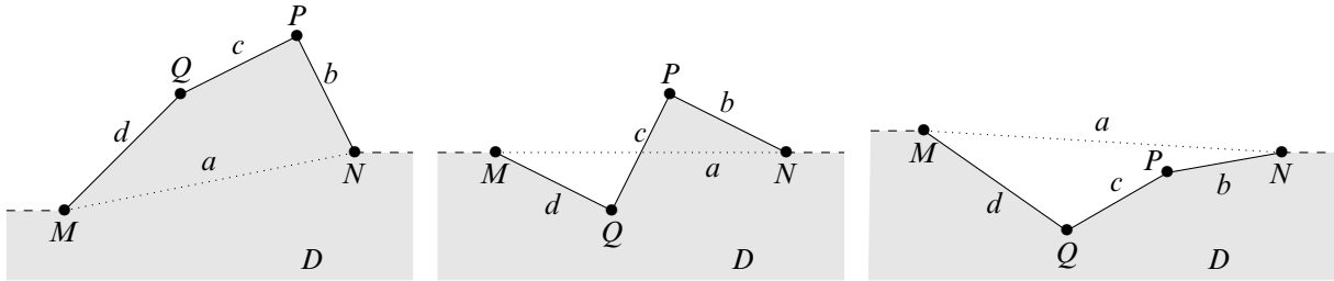
Figure 1: The disk D and the quadrilateral Q in three configurations.
