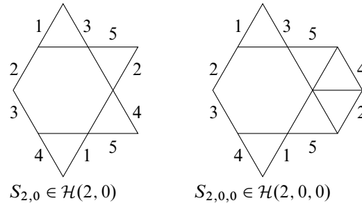
Figure 3: Local but nonglobal maxima in \mathcal{H}(2, 0) and \mathcal{H}(2, 0, 0) .
