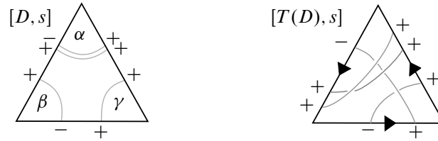
Figure 1: A stated diagram [D, s] in the triangle and its associated stated tangle [T(D), s] . Here, we use the order \gamma < \beta < \alpha . Here s is \sigma -increasing so [T(D), s] \in \mathcal{TB}^\sigma .
