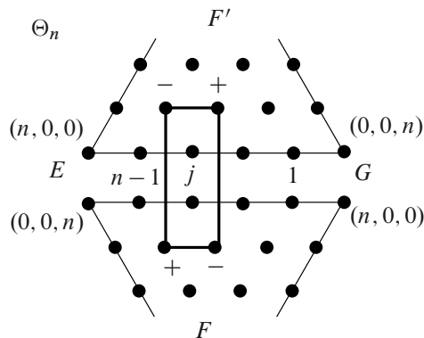
Figure 2: Edge invariants for a generic flag quadruple.
