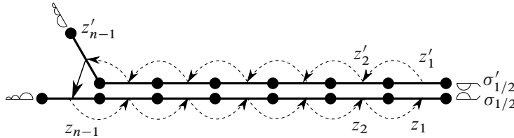
Figure 18: Right tail snake-move algebra for j = 1 .
