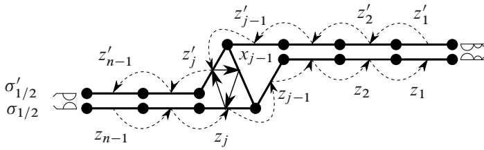
Figure 13: Diamond snake-move algebra for j = 2, \dots, n - 1 .
