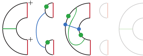
Figure 13: In S_2 , the specified endpoints cannot be connected by disjoint sorting arcs, so the foliated open book is not sorted.
