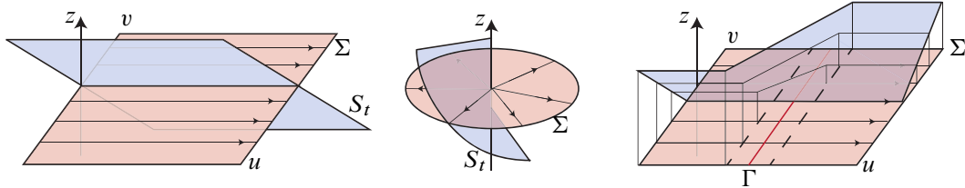
Figure 8: Local models for the open book of Lemma 4.4. The blue surfaces are pages of (B, \pi) , while the red surfaces are fibers \Sigma \times \{t\} . The model near a hyperbolic point, which is not shown, is a blue hyperboloid intersecting a horizontal red plane.
