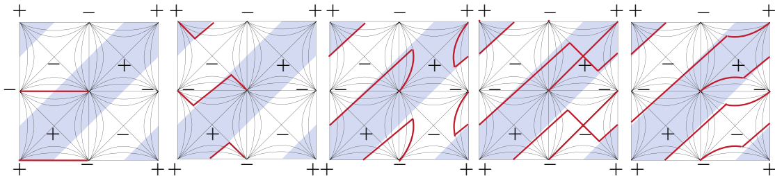
Figure 10: The red curves indicate how the page (\pi')^{-1}(0) intersects selected surfaces \Sigma \times \{t\} when Proposition 4.3 is applied to the foliated torus from Figure 1. On each surface \Sigma \times \{t\} , the blue region is R_+ and the white region is R_- . The t -values shown lie in [0, \frac{1}{2}] .
