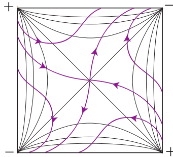
Figure 5: The flow of \nabla\tilde{\pi} on a tile.
