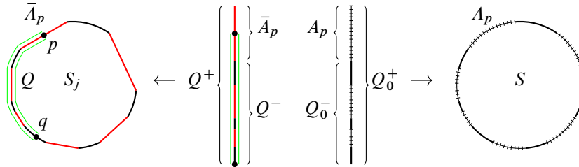
Figure 5: In the proof of Claim 4.13, from a geodesic segment Q of S_j (indicated by a green outline) we obtain Q^{-1} by removing the interiors of any \bar{Q}_i that are partially contained in Q . We obtain Q^+ \rightarrow S_j by extending the inclusion Q \hookrightarrow S_j to include full copies of any \bar{Q}_i that are partially contained in Q . From Q^- \hookrightarrow S_j and Q^+ \rightarrow S_j we obtain Q_0^- \hookrightarrow S and Q_0^+ \rightarrow S in S = S_0 by replacing any \bar{Q}_i \hookrightarrow S_j with Q_i \hookrightarrow S . The \bar{Q}_i with i < j are drawn in red in S_j . The Q_i with i < j are drawn with perpendicular markings in S .
