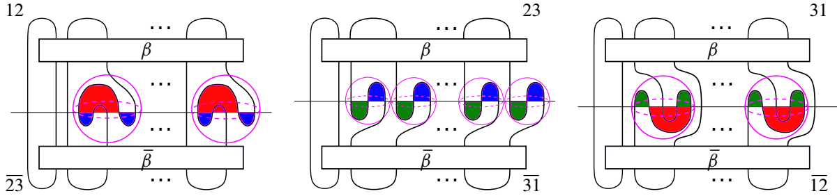
Figure 20: Bridge presentations for the links L_{\epsilon, \bar{\delta}} = T_\epsilon \cup \bar{T}_\delta .
