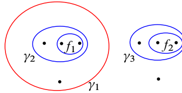
Figure 7: When the reducing curve bounds four punctures, the two cut curves lie on distinct sides.
