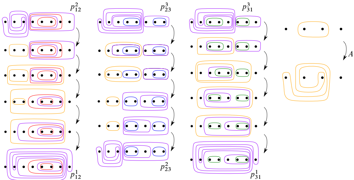
Figure 19: Three paths of length five between p_{ij}^i and p_{ij}^j .
