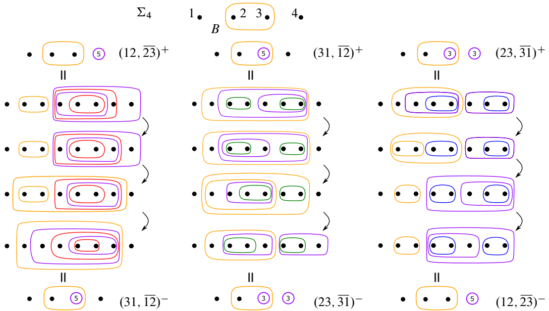
Figure 24: Paths of length three between G_{\epsilon, \delta}^+(p_1) and G_{\rho, \epsilon}^-(p_1) .
