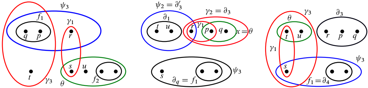
Figure 13: Curves interacting in the consecutive A -moves \gamma_1 \mapsto \theta , \gamma_n \mapsto \psi_n for a fixed n .
