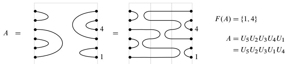
Figure 3: The set of innermost right cups of an element in \mathcal{TL}_6 .
