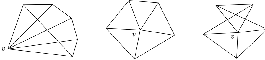
Figure 2: Typical vertex with positive (left), zero (middle), and negative (right) index.
