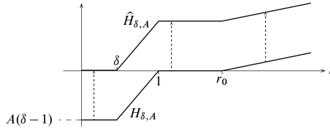
Figure 10: Homotopy from H_{\delta,A} to \hat{H}_{\delta,A} .
