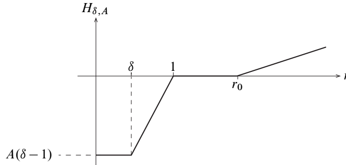
Figure 8: Radial portion of the Hamiltonian H_{\delta,A} .
