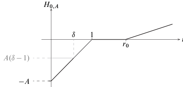
Figure 14: The continuous Hamiltonian H_{0,A} .
