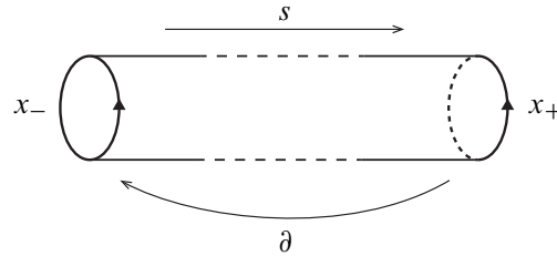
Figure 4: The differential in Floer cohomology goes from right to left.
