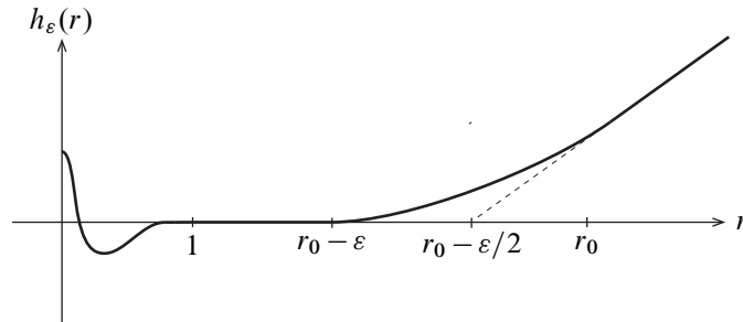
Figure 5: The \tau -extension of a compactly supported Hamiltonian.
