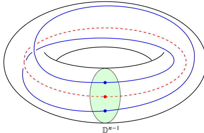
Figure 1: The local picture of the fibration in (5) near a singular point of \mathcal{O} . A nonsingular fiber (not dashed) winds m = 2 times around the singular fiber (dashed).
