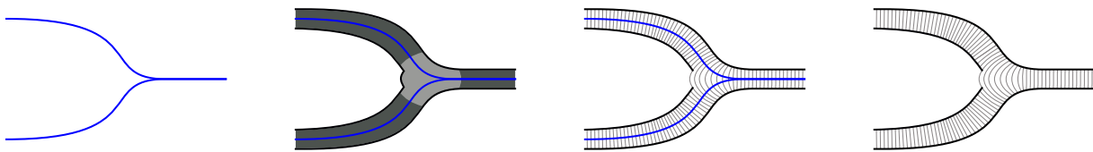
Figure 14: Constructing a train track \tau_i from the train graph T_i .
