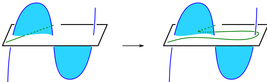
Figure 2: Bridge disks below \Sigma_K can be isotoped to intersect D_+^1 in two points in K .
