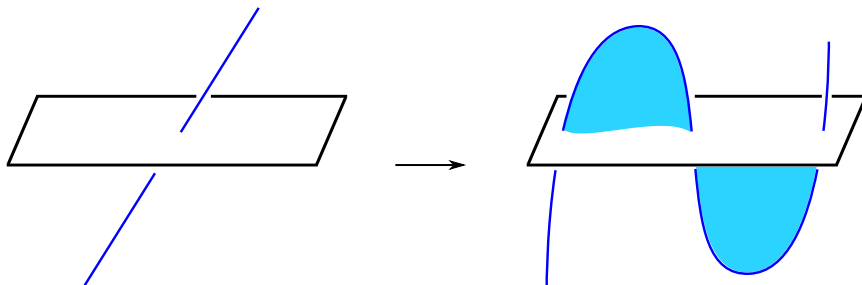
Figure 1: Introducing a canceling pair of critical points.
