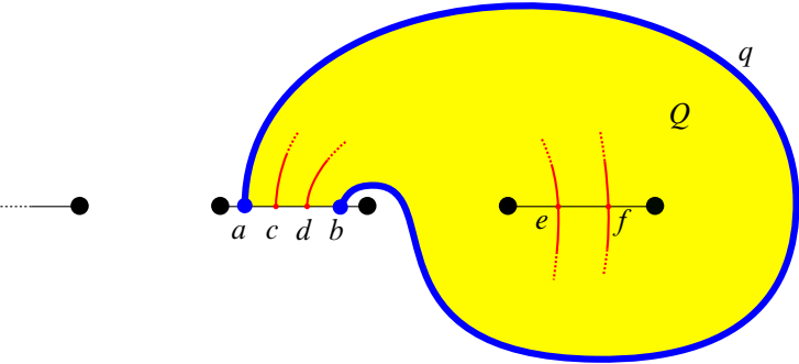
Figure 25: The arc q and the disk Q .
