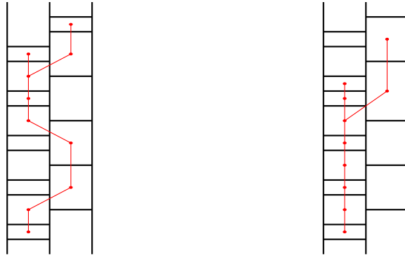
Figure 11: Subtrees of \sigma_1^2\sigma_2\sigma_1^2\sigma_2\sigma_1^2\sigma_2\sigma_1^2\sigma_2\sigma_1^2\sigma_2^2 and \sigma_1^2\sigma_2\sigma_1^2\sigma_2\sigma_1^2\sigma_2\sigma_1^3\sigma_2\sigma_1^2\sigma_2 .
