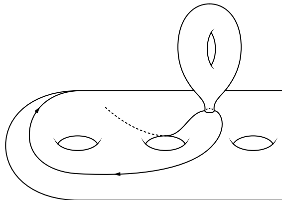
Figure 2: Point pushing (or rather, “small circle pushing”) the genus-one surface S^\beta along S_G/S_G^\beta .
