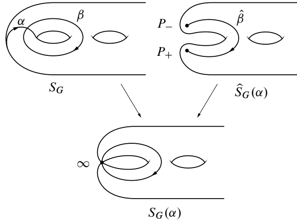
Figure 1: The surface S_G , its quotient S_G(\alpha) and the normalization \hat{S}_G(\alpha) .
