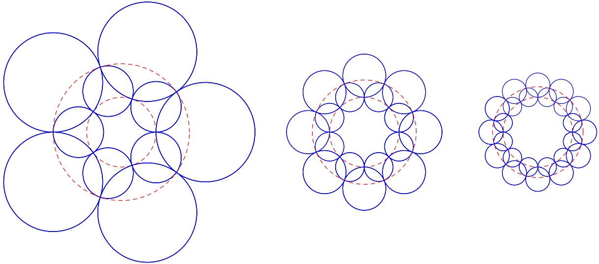
Figure 7: A visual proof that the distance between the “top” and “bottom” faces of the antiprism A_n approaches 0. Drawn above are the ideal boundaries of the walls of A_n for n = 5, 8, and 12 (from left to right), visualized via stereographic projection onto the page from the ideal boundary of \mathbb{H}^3 such that the circles corresponding to the top and bottom faces (the dashed circles) are concentric. Keeping fixed the Euclidean diameter of the inner dashed circle, as n approaches \infty the diameter of an inner solid circle approaches 0, so that the ratio between the diameters of the inner and outer dashed circles approaches 1. In fact, an elementary exercise in Euclidean geometry shows that this ratio is precisely (1 + \sin(\pi/n)) / \cos(\pi/n) , corroborating a computation of Kellerhals [16, Examples 1 and 2].
