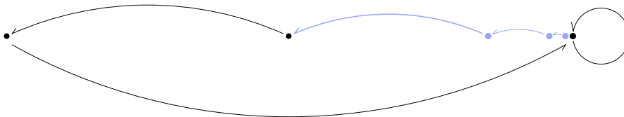
Figure 1: The forward orbit P(0) for the map f: z \rightarrow z^2 - 2 is in black, and the tail T is in blue (gray) (only three elements of T are shown in the figure).
