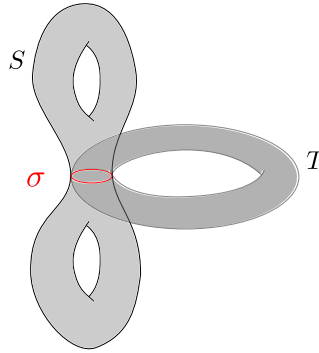
Figure 14: A homotoped elementary drilled atom.
